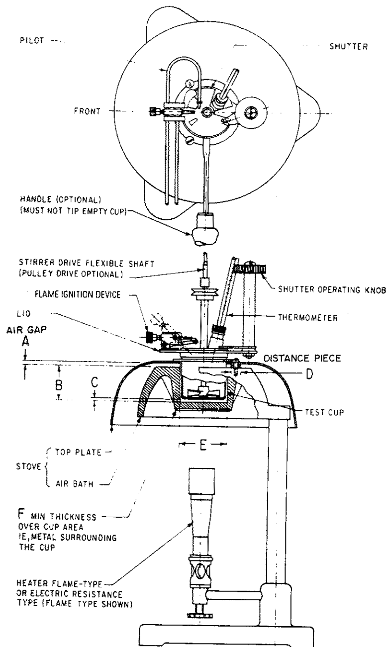
FIG. A1.1 Pensky-Martens Closed Flash Tester
